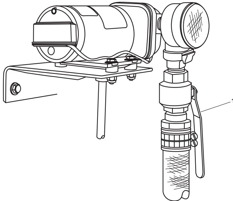
Figure 14. Fresh Water Flush Pump Outlet Valve
