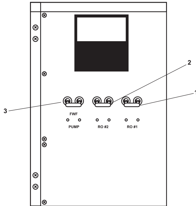
Figure 5. ROWPU 24 Vdc Control Panel
