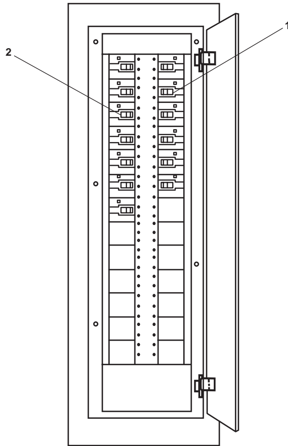
Figure 6. 440V Power Panel No. 5
