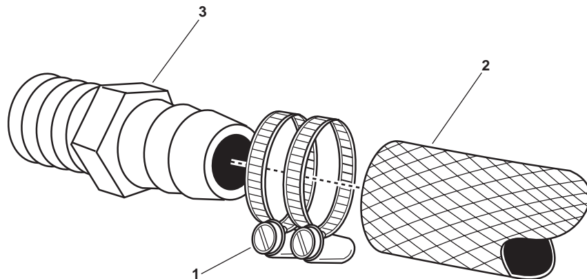
Figure 1. Low Pressure Fitting, Hose, and Clamp
