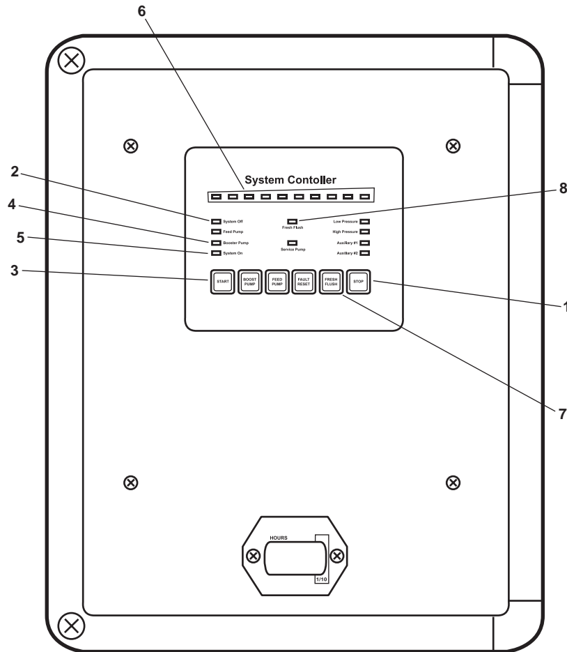
Figure 13. System Controller
