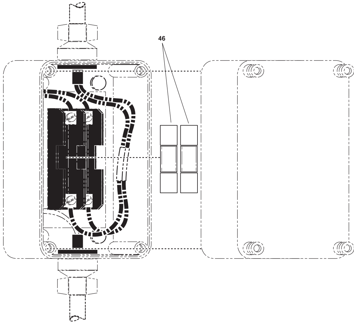
24 Vdc Fuse Box
