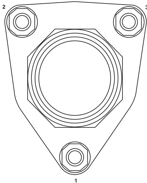
Figure 2. Torque Pattern for Sil Braze Ball Valve
