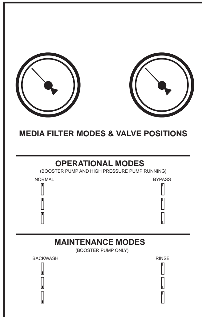
Figure 12. Media Filter Maintenance Mode Valve Positions
